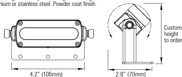
Custom height IP66 adjustable angle mounting bracket Aluminium or stainless steel. Powder coat finish.
