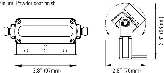
Standard IP66 adjustable angle mounting bracket Aluminium. Powder coat finish.
